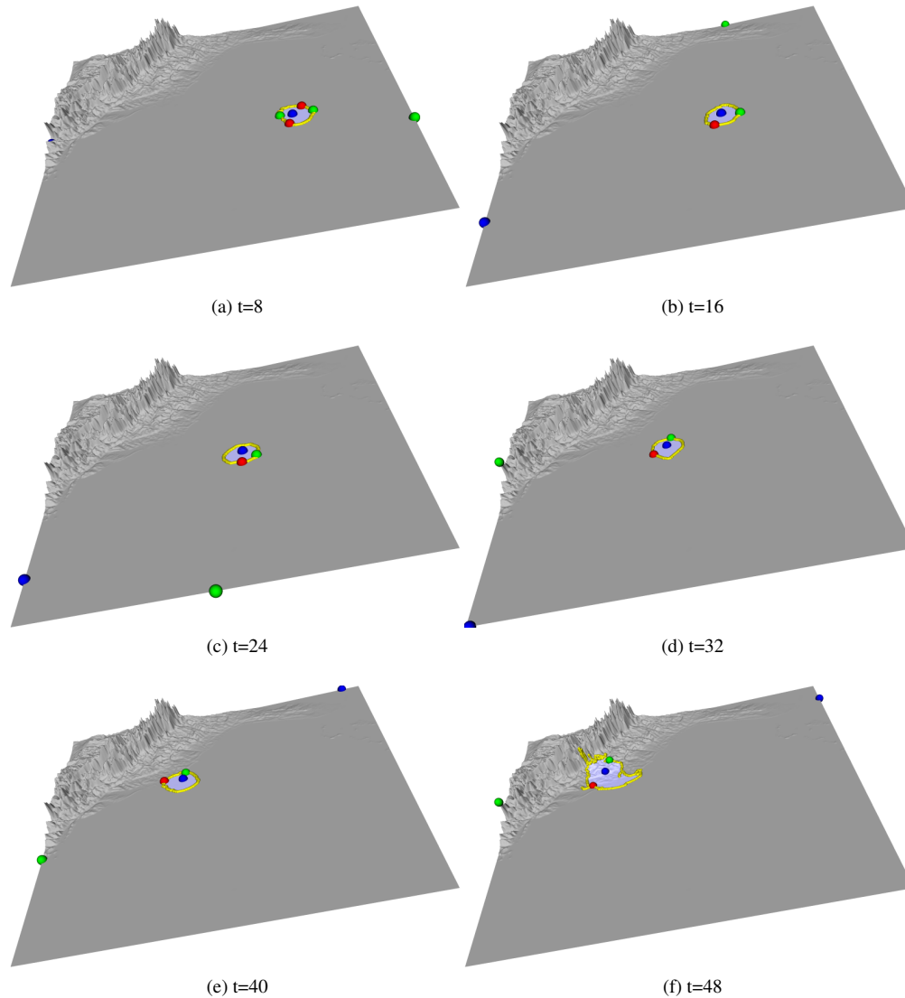
Figure 1: The ascending manifold of the most persistent wind speed minimum corresponds to the eye of the hurricane. Computing this ascending manifold tracks the eye. Since the wind velocity drops sharply at the eye of the hurricane and increases sharply around the eye, the gradient behavior of the magnitude captures the movement of hurricane. The images show the MS complex of the wind speed above the surface, rendered onto the surface height field for every 8 th time step beginning from the 8 th . The MS complexes for (a),(b),(c),(d) were simplified upto 20%. (e) and (f) were simplified upto 25% and 35% respectively.
