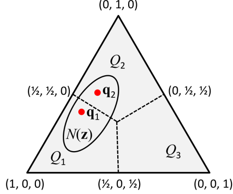
Figure 4: Visual proof of Theorem 6. If a surrogate \psi is such that its positive normal set \mathcal{N}^\psi(\mathbf{z}) at some point \mathbf{z} has non-empty intersection with the interiors of two trigger probability sets (say \mathcal{Q}_1^{\mathbf{L}} and \mathcal{Q}_2^{\mathbf{L}} ) of \mathbf{L} , then \psi cannot be \mathbf{L} -calibrated.
