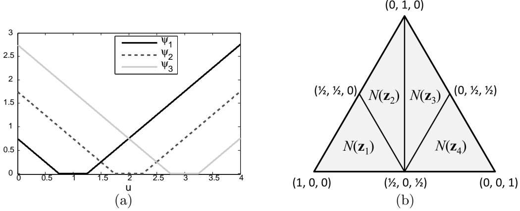
Figure 6: (a) The ‘ \epsilon -insensitive’ surrogate \psi^\epsilon : \mathbb{R} \rightarrow \mathbb{R}_+^3 for \epsilon = 0.25 (and n = 3 ), and (b) its positive normal sets at 4 points \mathbf{z}_i = \psi^\epsilon(u_i) \in \mathbb{R}_+^3 ( i \in [4] ) for u_1 = 1.25, u_2 = 1.75, u_3 = 2.25, u_4 = 2.75 . See Example 9 for details.
