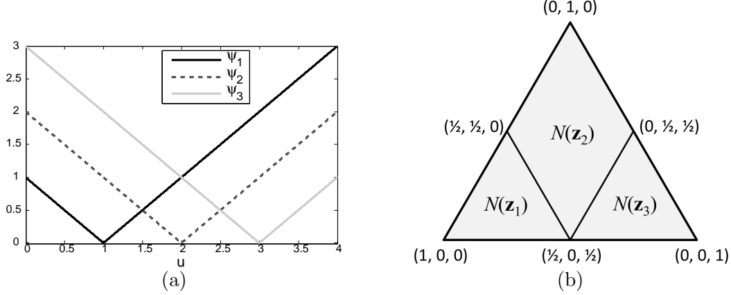
Figure 5: (a) The ‘absolute’ surrogate \psi^{\text{abs}} : \mathbb{R} \rightarrow \mathbb{R}_+^3 (for n = 3 ), and (b) its positive normal sets at 3 points \mathbf{z}_i = \psi^{\text{abs}}(u_i) \in \mathbb{R}_+^3 ( i \in [3] ) for u_1 = 1, u_2 = 2, u_3 = 3 . See Example 8 for details.
