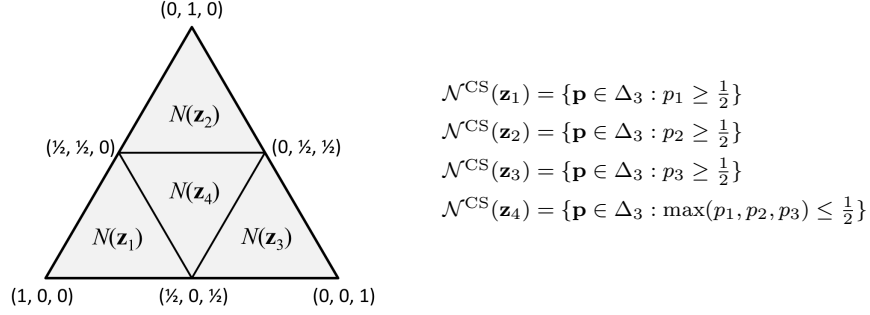
Figure 3: Positive normal sets for the Crammer-Singer surrogate \psi^{\text{CS}} for n = 3 , at 4 points \mathbf{z}_i = \psi^{\text{CS}}(\mathbf{u}_i) \in \mathbb{R}_+^3 ( i \in [4] ) for \mathbf{u}_1 = (1, 0, 0)^\top , \mathbf{u}_2 = (0, 1, 0)^\top , \mathbf{u}_3 = (0, 0, 1)^\top , and \mathbf{u}_4 = (0, 0, 0)^\top . Calculations of these sets are based on Lemma 9 and can be found in Appendix C.
