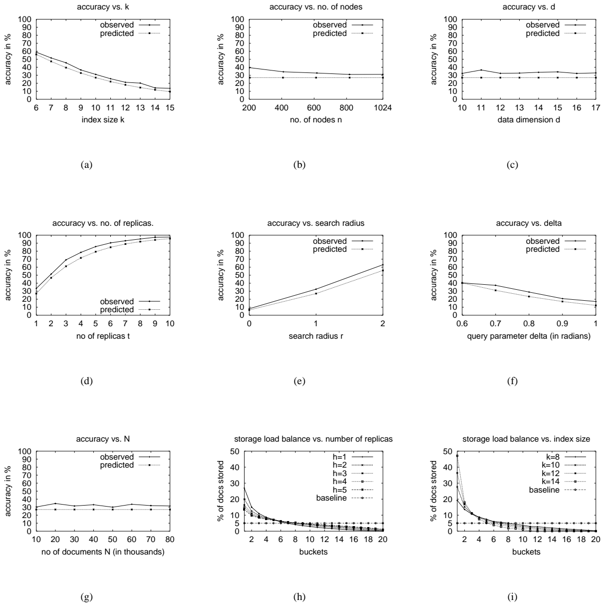
Figure 1. Experimental Results for Accuracy and Storage Load Balance
