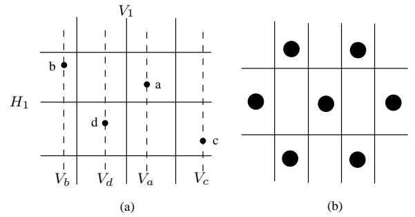
Figure 4: Upper and Lower bounds for \epsilon_4^{\mathcal{R}}
