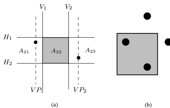
Figure 2: Upper and lower bounds for \epsilon_2^{\mathcal{R}}
