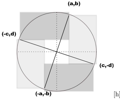
Figure 7: To prove Lemma 11
